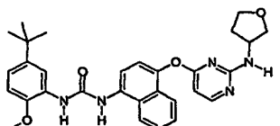
1-(5-tert-Butyl-2-methoxy-phenyl)-3-{4-[2-(tetrahydro-furan-3-ylamino)-pyrimidin-4-yloxy]-naphthalen-1-yl}-urea;
